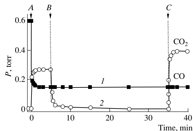
Fig. 6. Oxidation of CO with \alpha -oxygen over FeZSM-5 zeolite surface at 100°C (A is the instant of opening the microreactor; B is the beginning of freezing; and C is the beginning of thawing the trap): (1) the amount of CO and (2) the amount of \text{CO}_2 .
