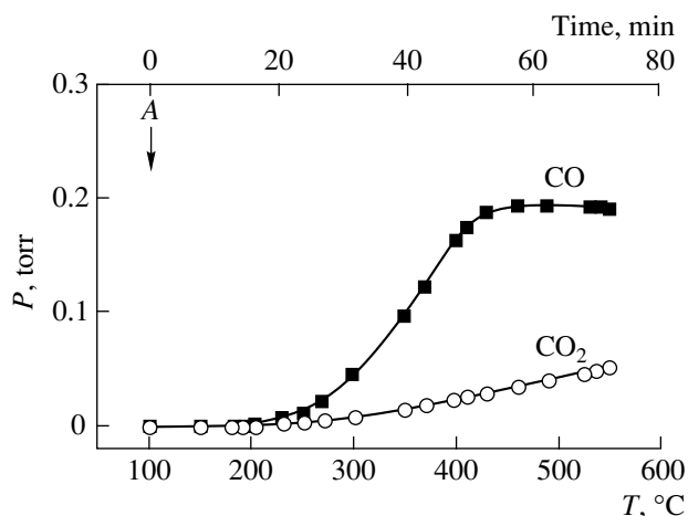
Fig. 2. Temperature-programmed desorption of the product of the oxidation of CH_4 by \alpha -oxygen ( A is the beginning of thawing).
