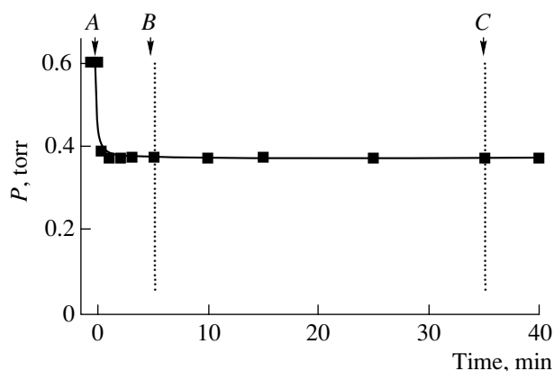
Fig. 1. Oxidation of CH_4 by \alpha -oxygen over the FeZSM-5 zeolite surface at 100^\circ C ( A is the instant of opening the microreactor; B is the beginning of freezing; and C is the beginning of thawing the trap).
