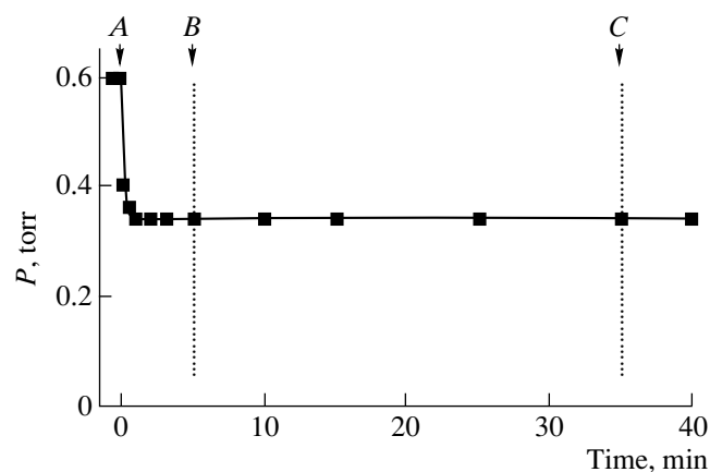
Fig. 3. Oxidation of D_2 by \alpha -oxygen over the FeZSM-5 zeolite surface at 100^\circ C (A is the instant of opening the microreactor; B is the beginning of freezing; and C is the beginning of thawing the trap).
