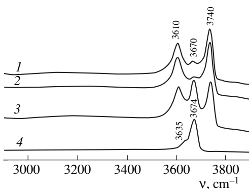
Fig. 7. IR spectra of FeZSM-5 zeolite in the region of OH vibrations recorded (1) after the standard treatment of the zeolite, (2) after the formation of \alpha -oxygen on the zeolite surface; (3) after the reaction between H_2 and \alpha -oxygen; and (4) after subtracting spectrum 1 from spectrum 3 (the difference spectrum).
