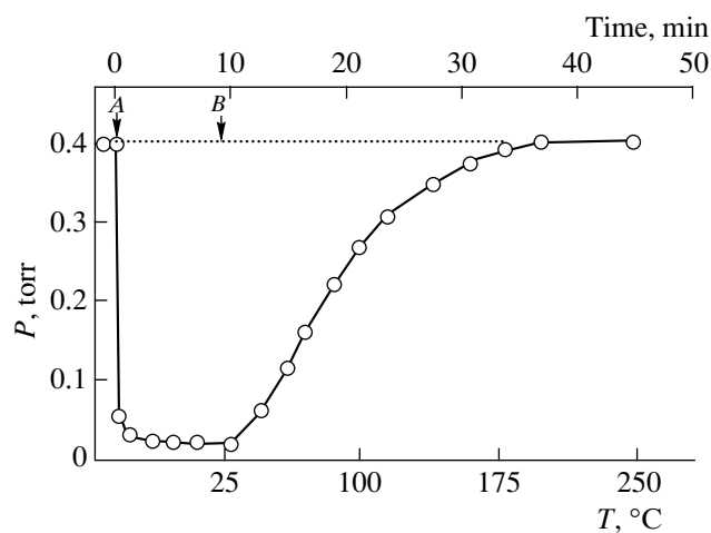
Fig. 4. Temperature-programmed desorption of CO_2 from the FeZSM-5 zeolite surface (A is the instant of opening the microreactor and admitting CO_2 and B is the beginning of thawing).
