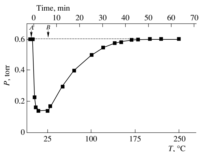
Fig. 5. Temperature-programmed desorption of CO from the FeZSM-5 zeolite surface (A is the instant of opening the microreactor and B is beginning of thawing).
